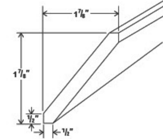
Decorative Moulding
